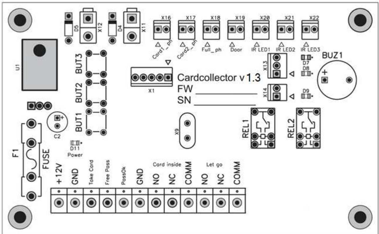
Fig. 16 General view of board
