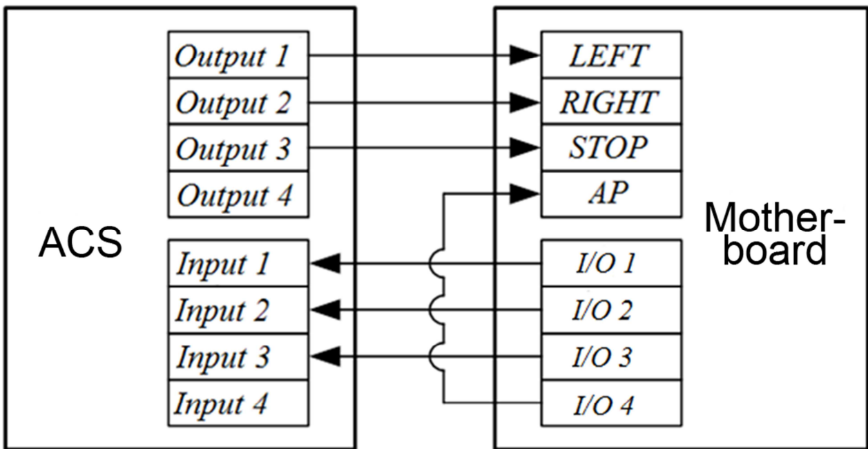
Fig. 14 Connection pattern of RC panel to ACS controller
