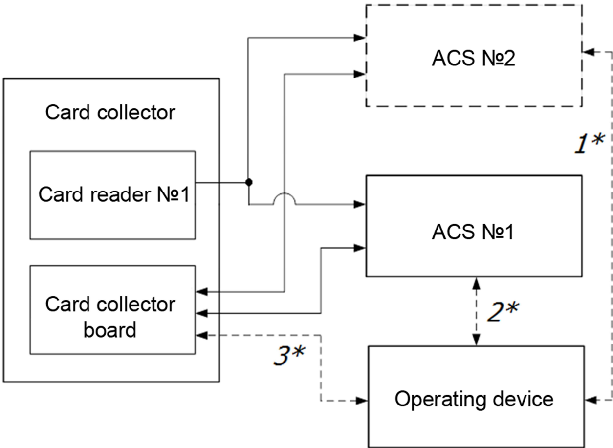
Fig. 21 Block diagram №2
