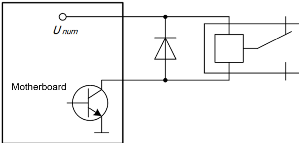
Fig. 13 Connection of diode in parallel with the relay coil
