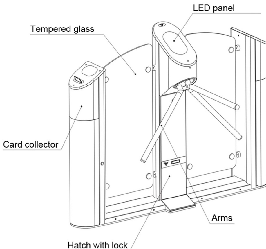
Fig. 1 General view of turnstile
