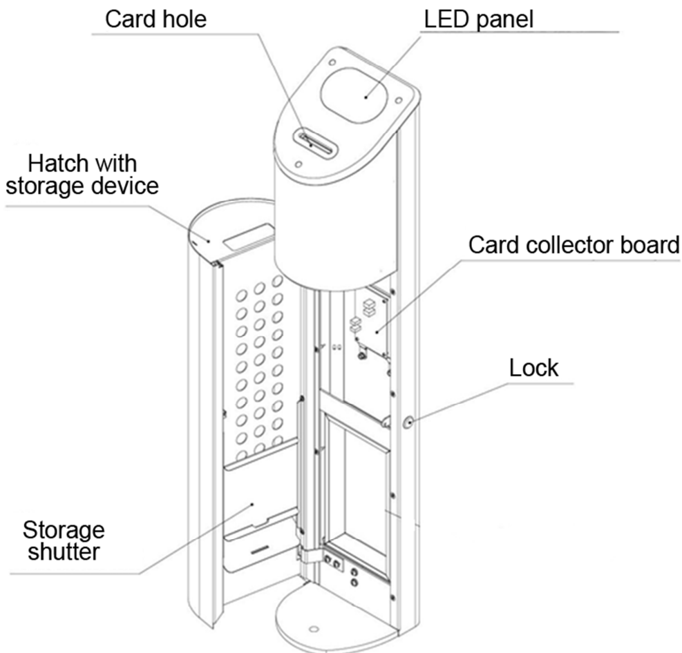
Fig. 15 General view of card collector
