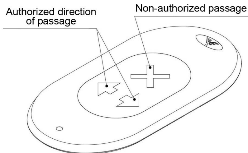
Fig. 4 General view of display panel
