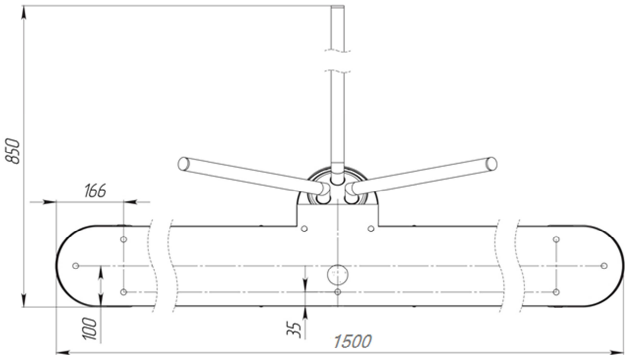
Fig. 23 Location of mounting holes in relation to the overall dimensions of the turnstile
