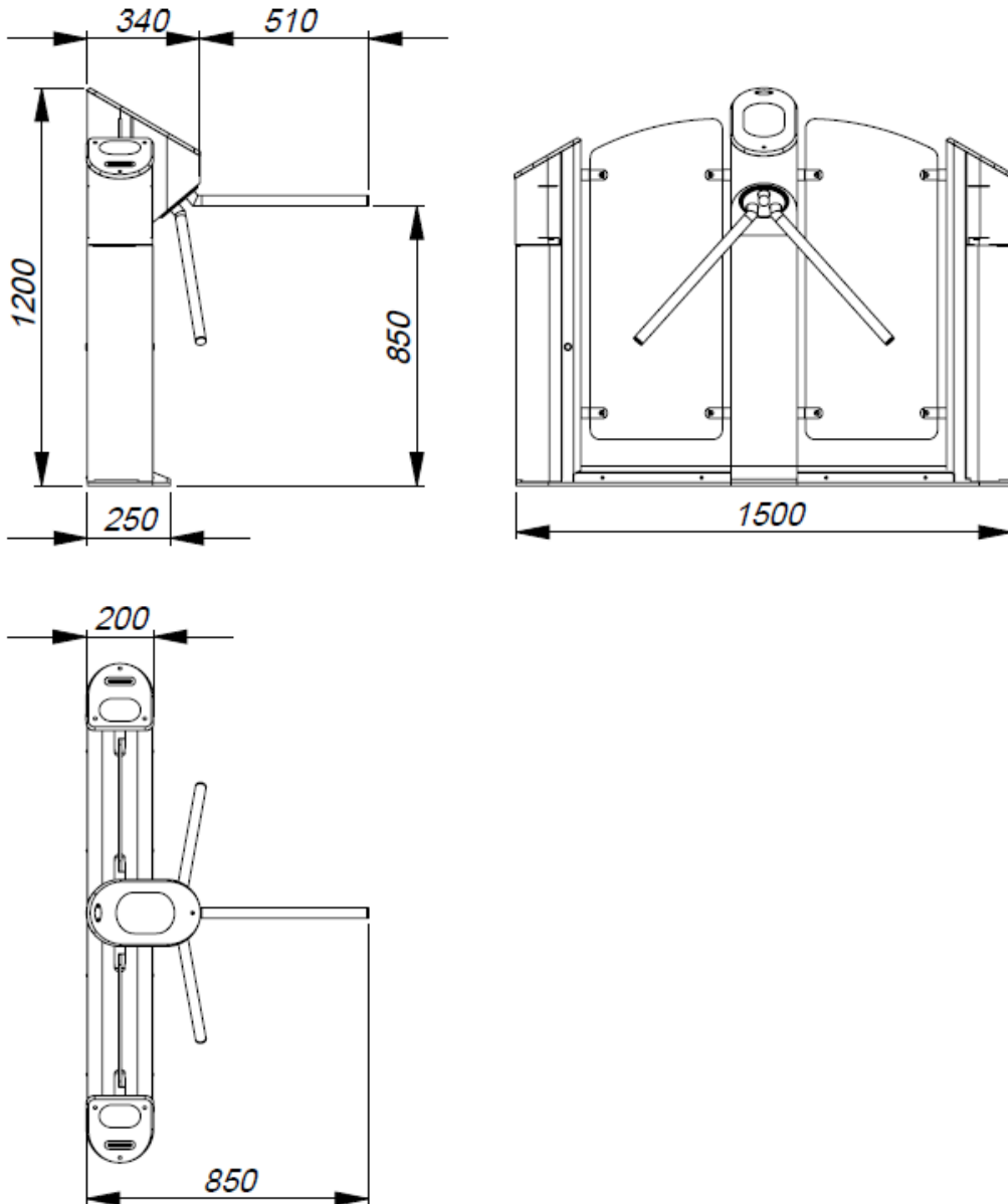
Fig 2. Dimensions of turnstile
